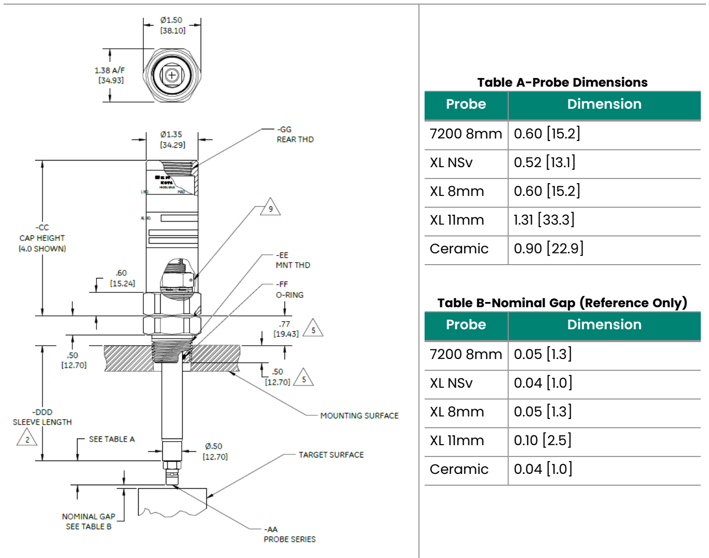
Figure 3: 164818 Compact Proximity Probe Housing
